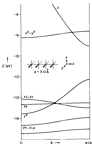
Fig. 3. Computed band structure of an eclipsed [\text{PtH}_4]^{2\ominus} stack, spaced at 3 Å. The orbital marked d_{xz} , d_{yz} is doubly degenerate.
