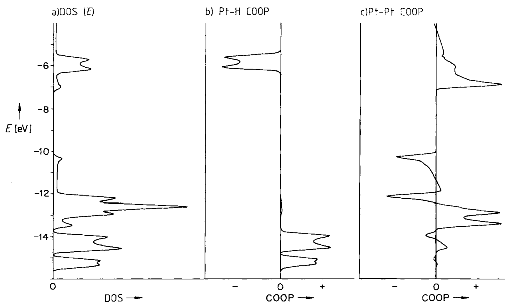
Fig. 9. Total density of states (a), and Pt-H (b) and Pt-Pt (c) crystal orbital overlap population curves for the eclipsed [\text{PtH}_4]^{2\ominus} stack.
