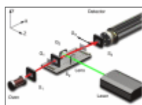
Figure 2 Layout of the Kapitza-Dirac-Talbot-Lau (KDTL) interference experiment.
