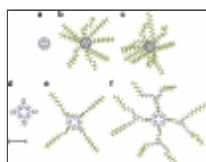
Figure 1 Gallery of molecules used in our interference study.
