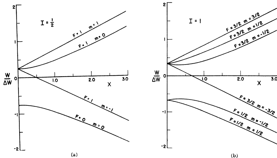
FIG. 1. The magnetic field dependence of the magnetic levels arising from the components of an h.f.s. doublet (a) for the case in which J = \frac{1}{2} , I = \frac{1}{2} (hydrogen) and (b) for the case in which J = \frac{1}{2} , I = 1 (deuterium). Each level is labeled by the quantum numbers F and m appropriate in the region of very weak magnetic field.
